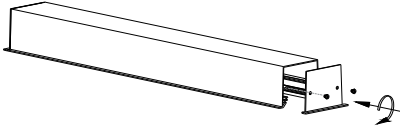
Gavel installation
