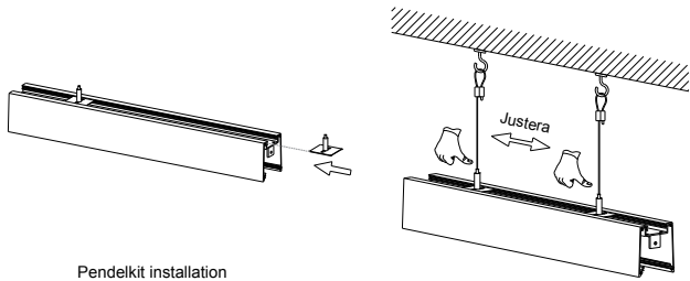
Pendelkit installation
