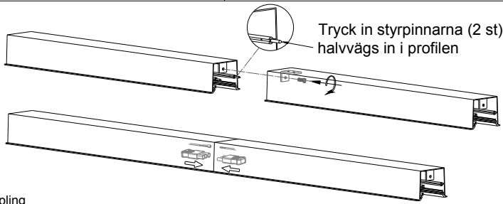
Profilkoppling
